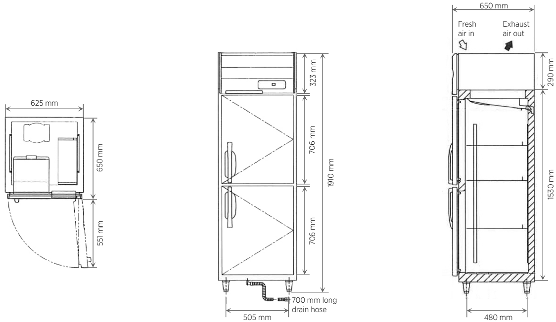
Upright Model with 625 mm Width
