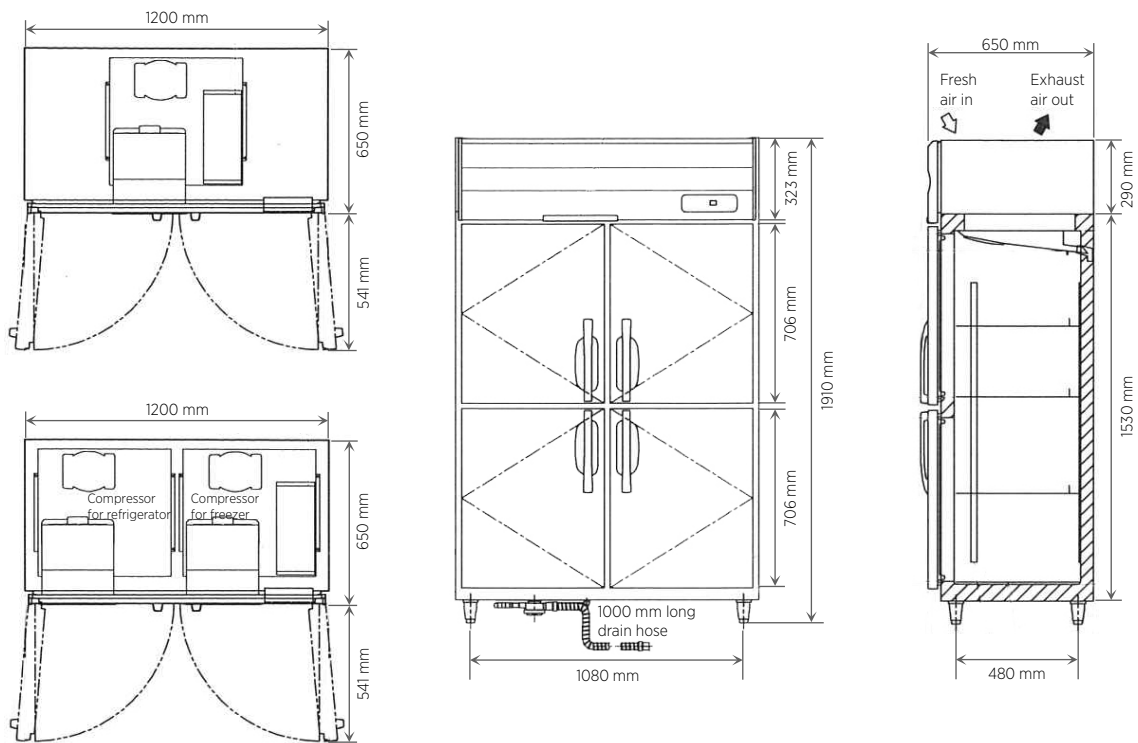
Upright Model with 1200 mm Width
